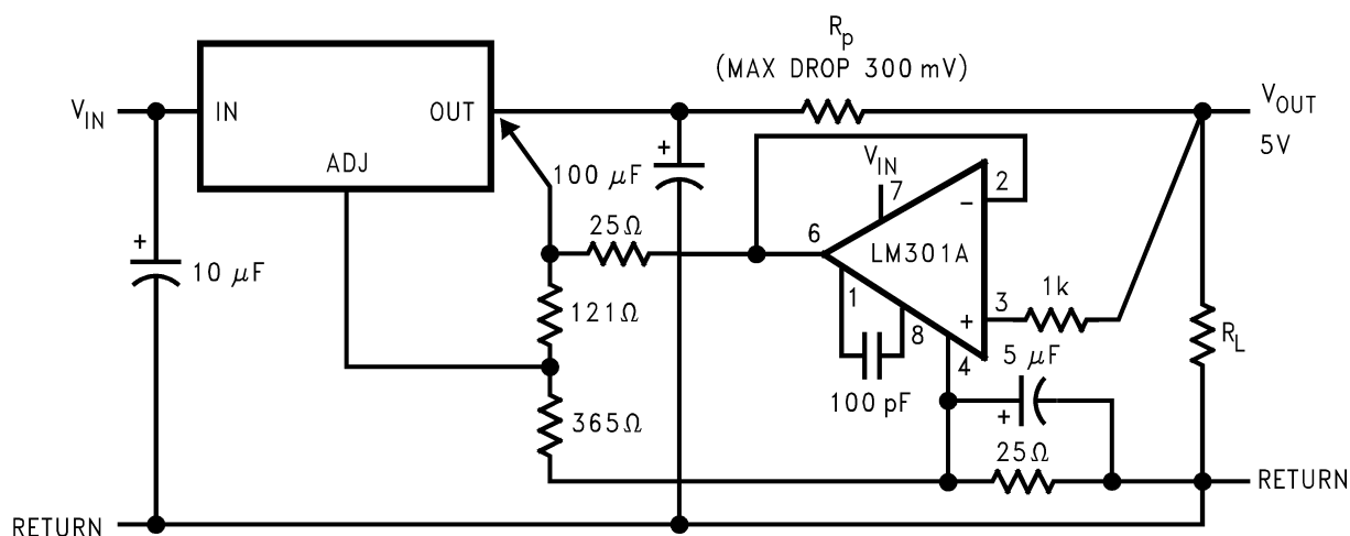
Figure 26. Remote Sensing
