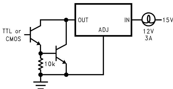
Figure 21. High Current Lamp Driver Protection
