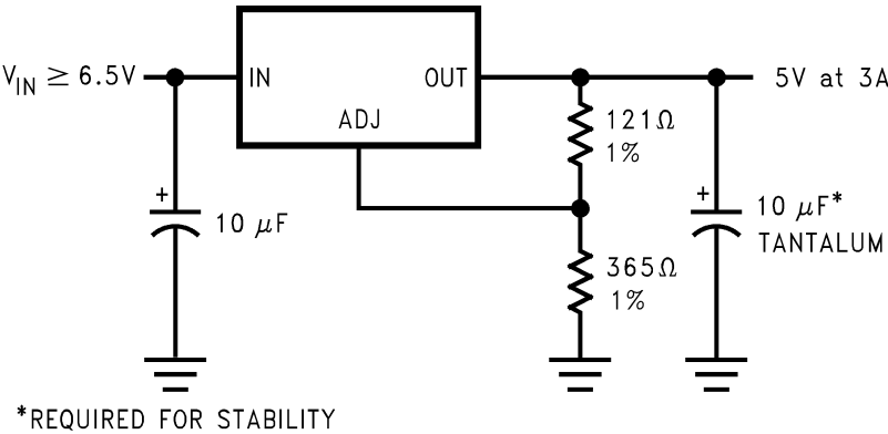
Figure 16. Adjustable @ 5V
