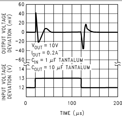
Figure 8. Line Transient Response
